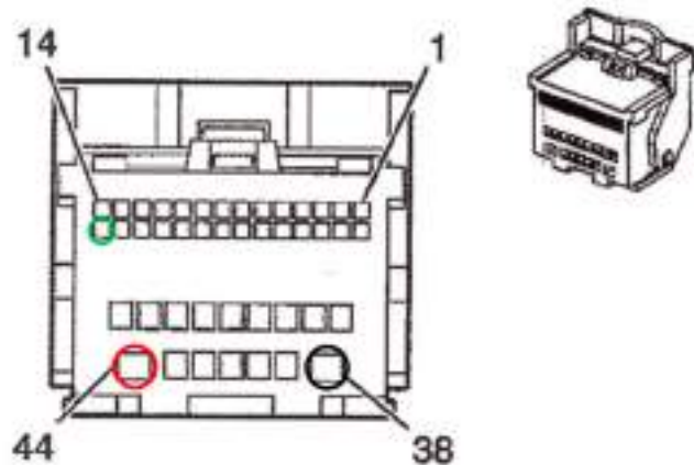
Pin definition female vehicle connector
